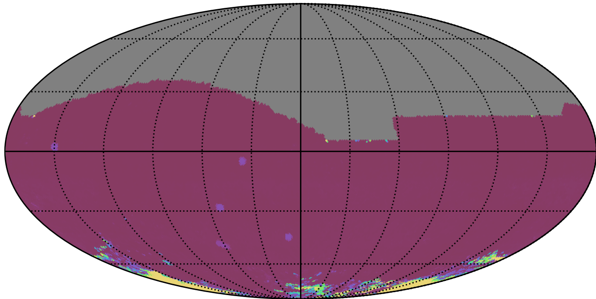
mw_roll_all_v3.3_10yrs All sky iz bands: 75th Percentile Intranight Timespan
