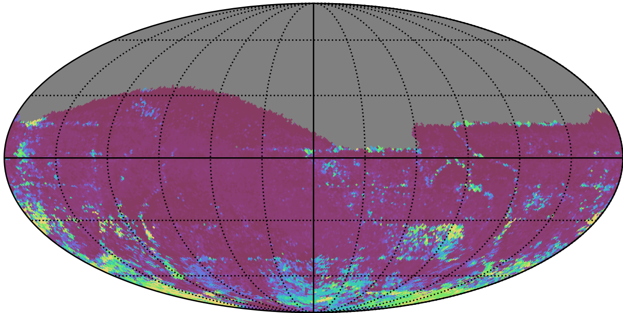
mw_roll_all_v3.3_10yrs All sky i band: 75th Percentile Intranight Timespan
