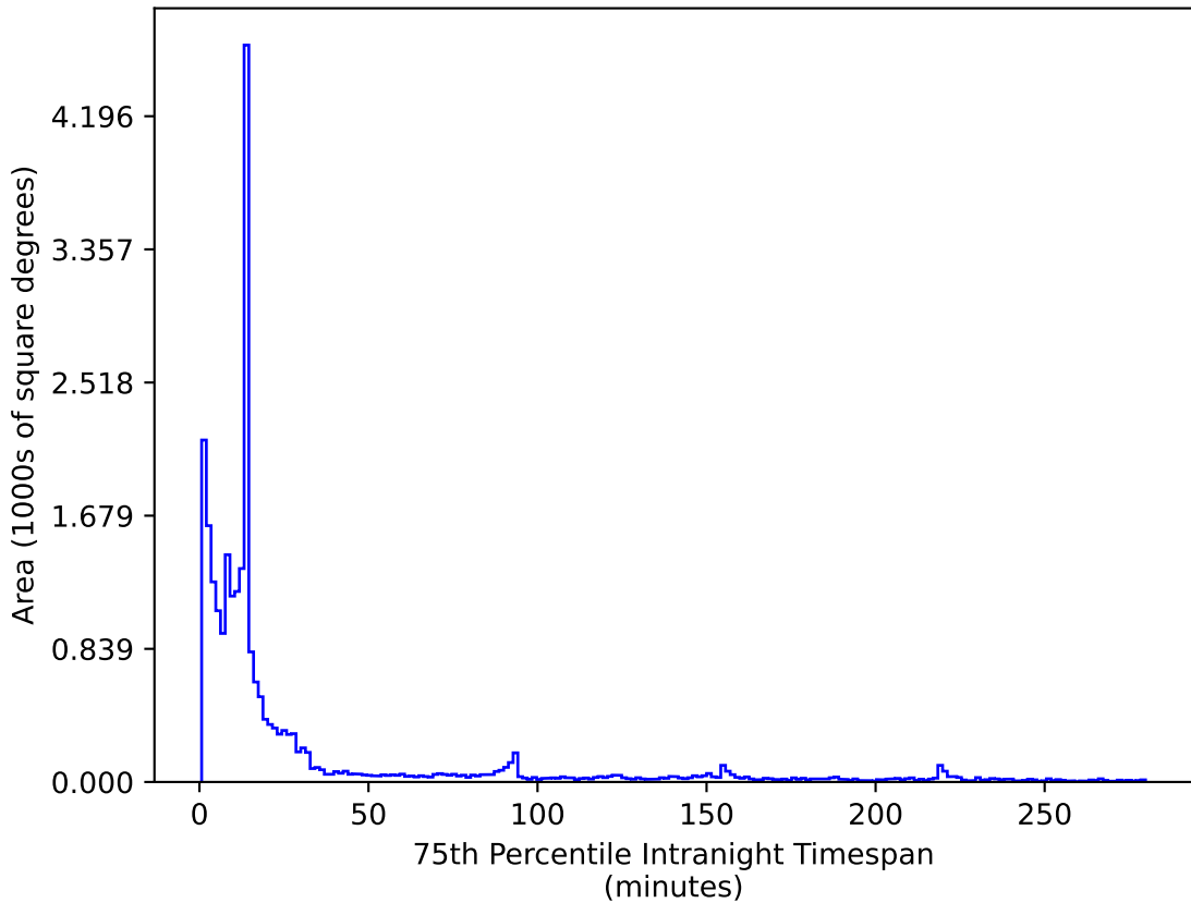
mw_roll_all_v3.3_10yrs All sky i band: 75th Percentile Intranight Timespan
