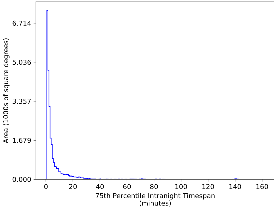
mw_roll_all_v3.3_10yrs All sky g band: 75th Percentile Intranight Timespan
