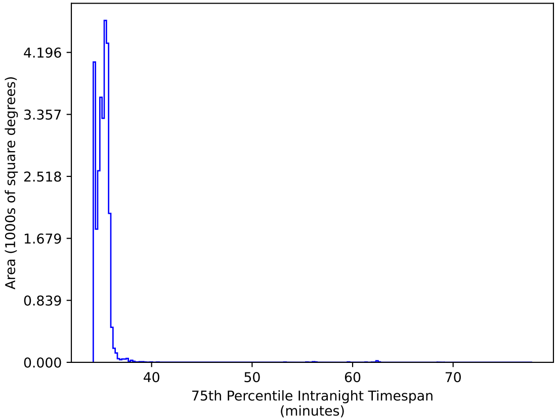
mw_roll_all_v3.3_10yrs All sky all bands: 75th Percentile Intranight Timespan
