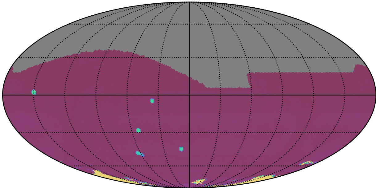
mw_roll_all_v3.3_10yrs All sky: 75th Percentile Intranight Timespan
