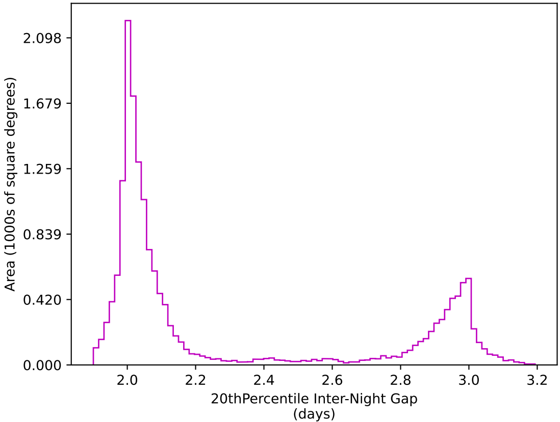
mw_roll_all_v3.3_10yrs WFD z band: 20thPercentile Inter-Night Gap
