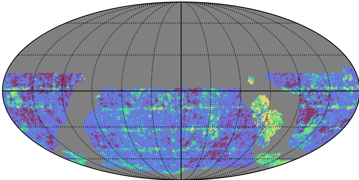
mw_roll_all_v3.3_10yrs WFD y band: 20thPercentile Inter-Night Gap
