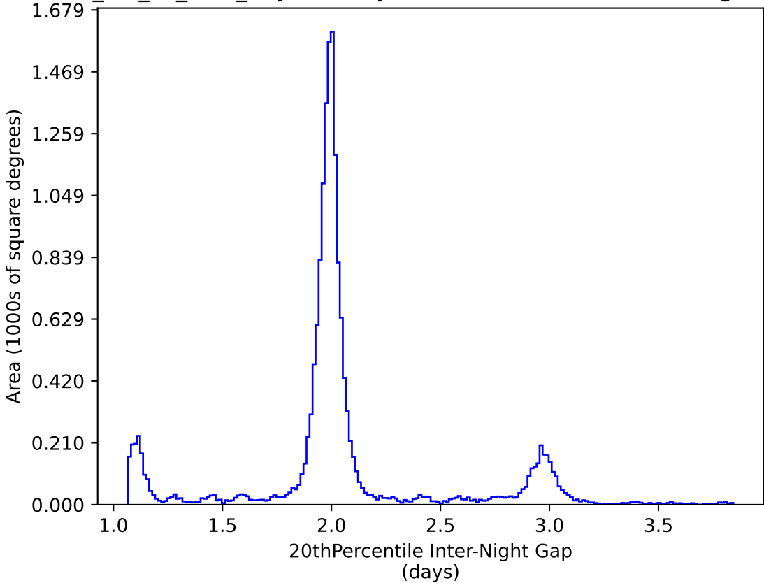
mw_roll_all_v3.3_10yrs WFD y band: 20thPercentile Inter-Night Gap
