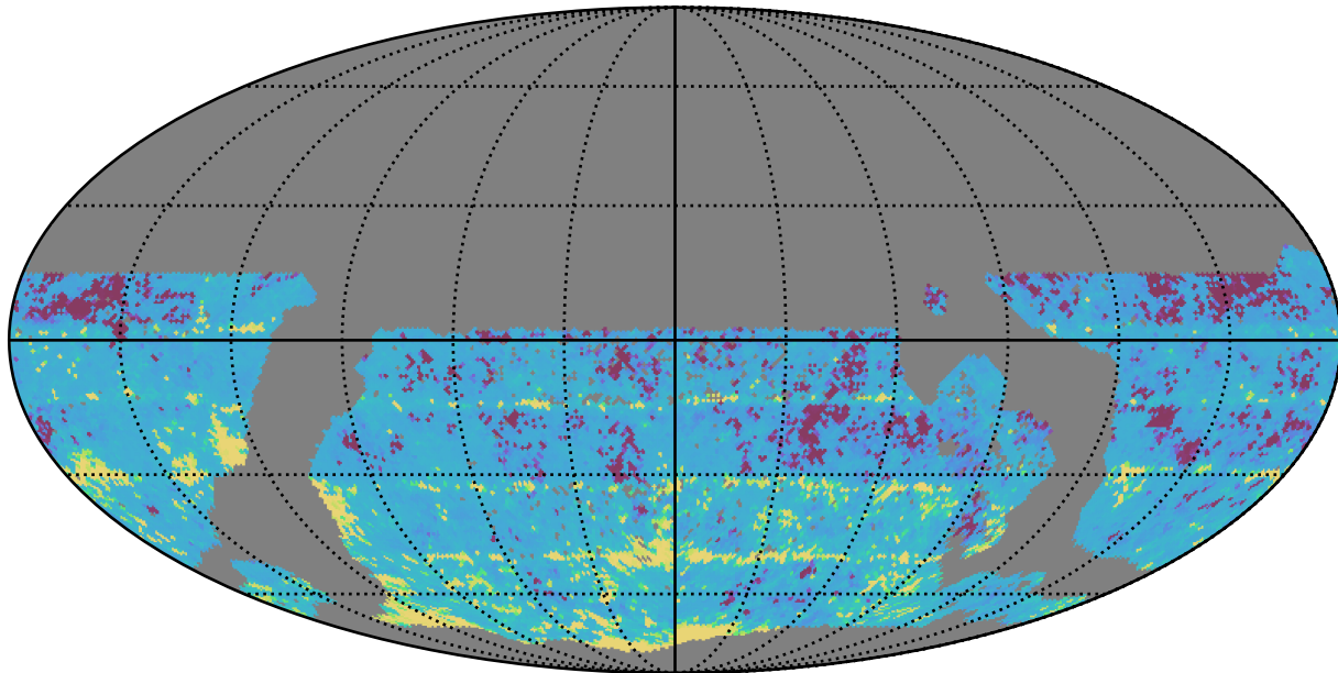
mw_roll_all_v3.3_10yrs WFD r band: 20thPercentile Inter-Night Gap
