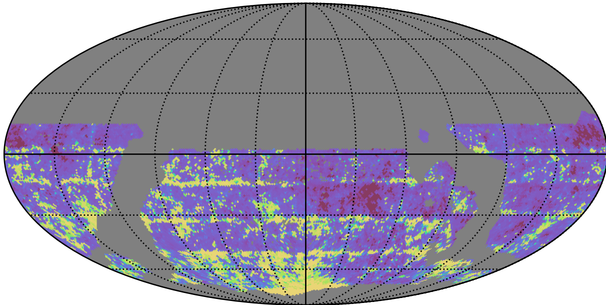
mw_roll_all_v3.3_10yrs WFD i band: 20thPercentile Inter-Night Gap
