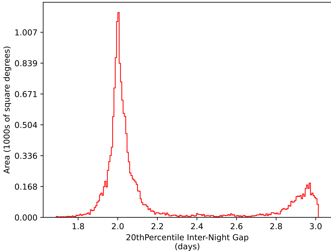
mw_roll_all_v3.3_10yrs WFD i band: 20thPercentile Inter-Night Gap
