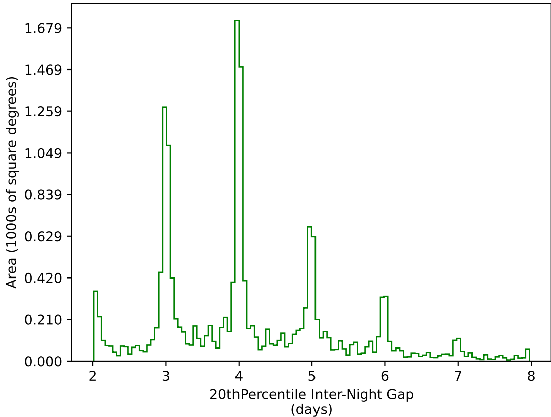
mw_roll_all_v3.3_10yrs WFD g band: 20thPercentile Inter-Night Gap
