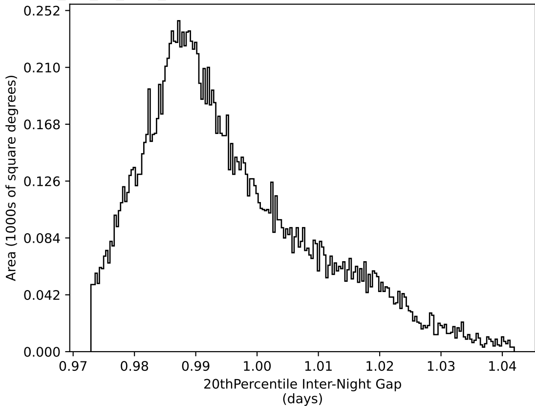
mw_roll_all_v3.3_10yrs WFD all bands: 20thPercentile Inter-Night Gap
