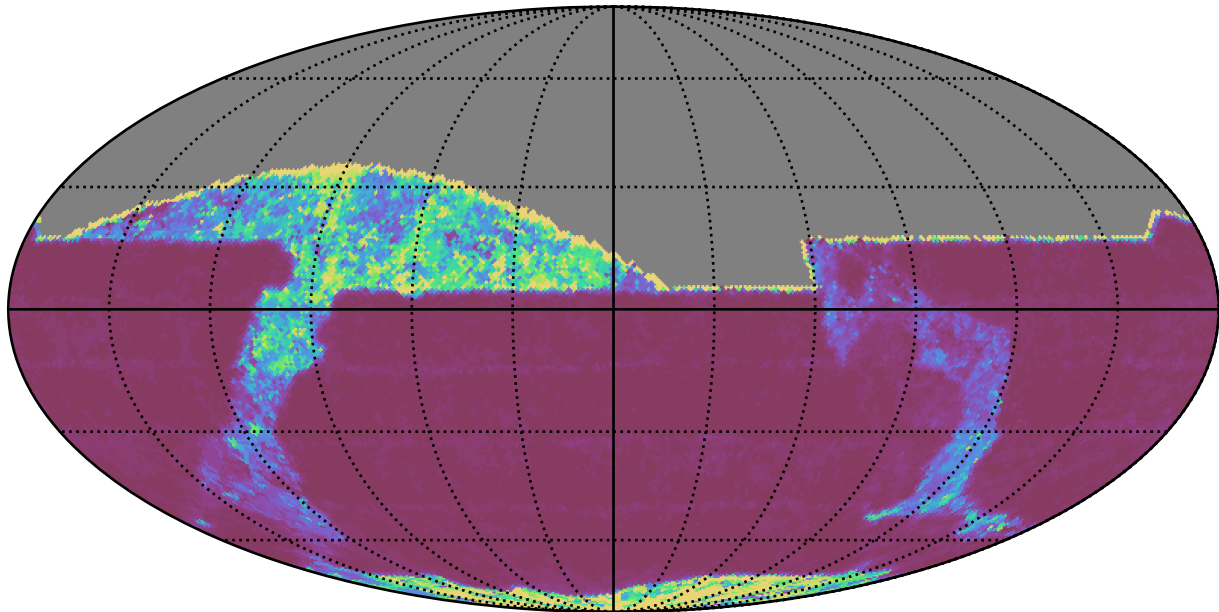
mw_roll_all_v3.3_10yrs All sky z band: 20thPercentile Inter-Night Gap
