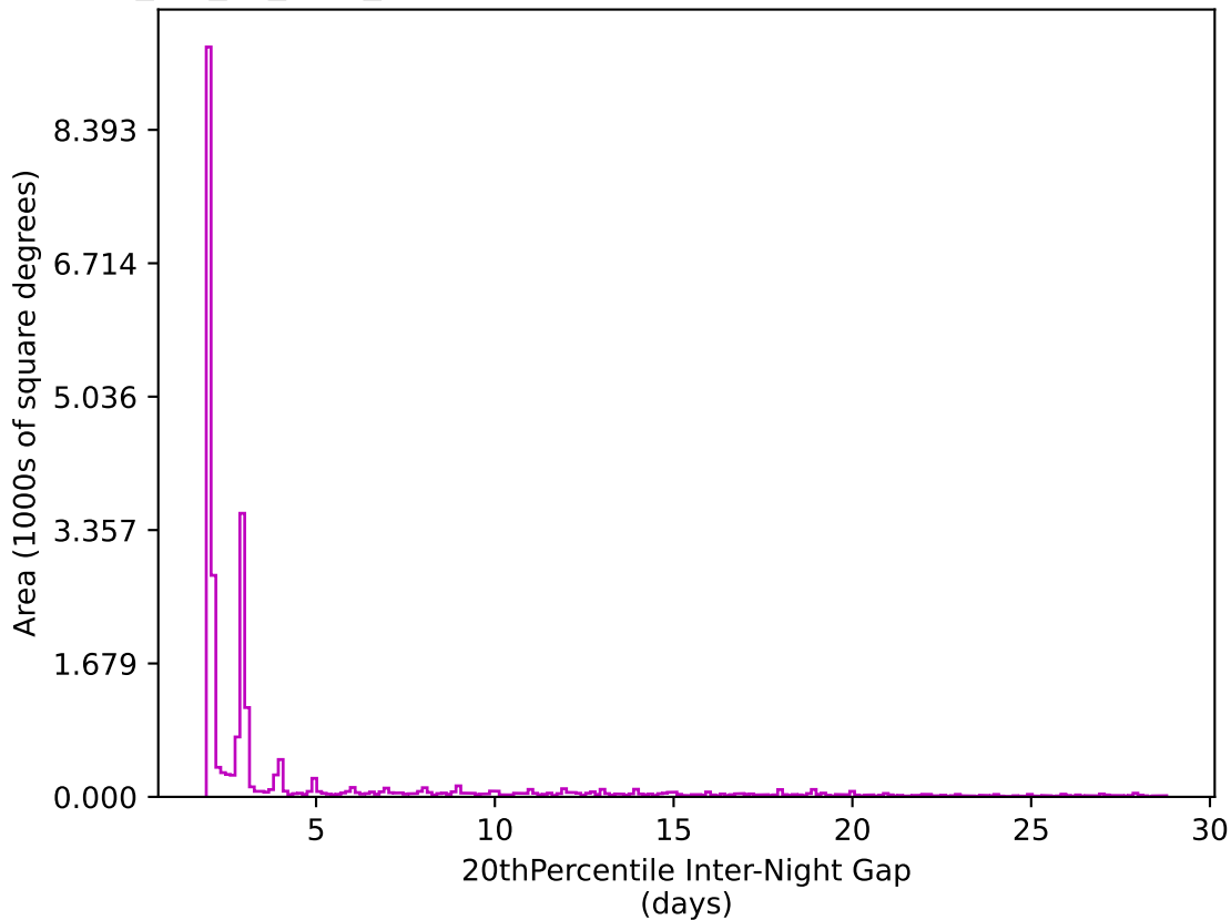
mw_roll_all_v3.3_10yrs All sky z band: 20thPercentile Inter-Night Gap
