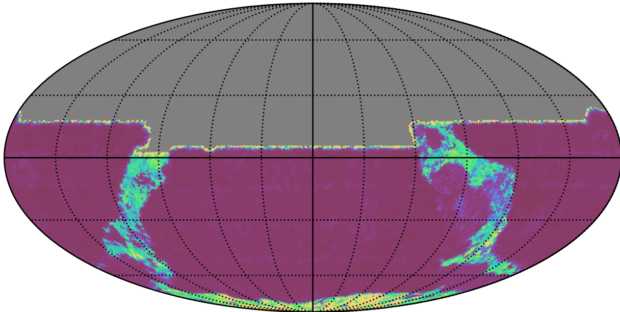
mw_roll_all_v3.3_10yrs All sky y band: 20thPercentile Inter-Night Gap
