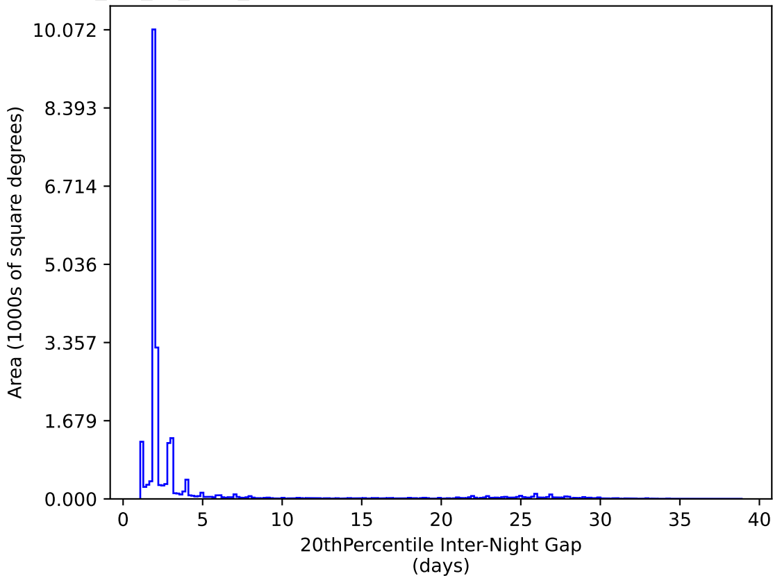
mw_roll_all_v3.3_10yrs All sky y band: 20thPercentile Inter-Night Gap
