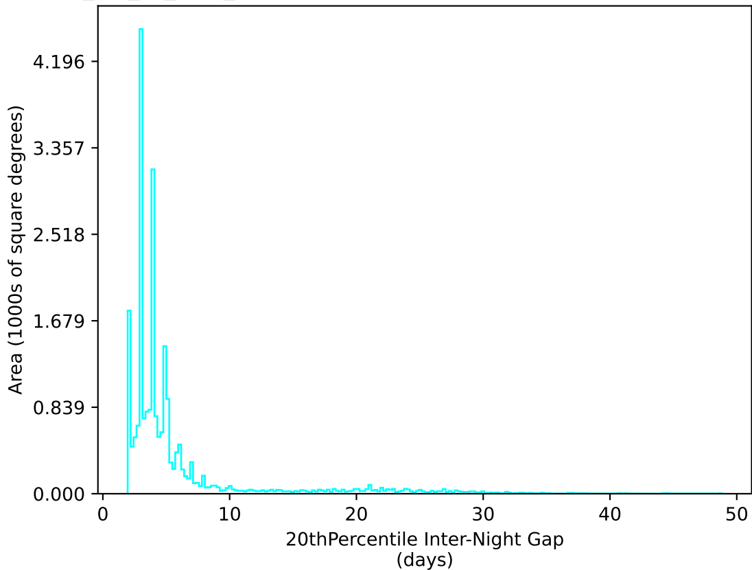
mw_roll_all_v3.3_10yrs All sky u band: 20thPercentile Inter-Night Gap
