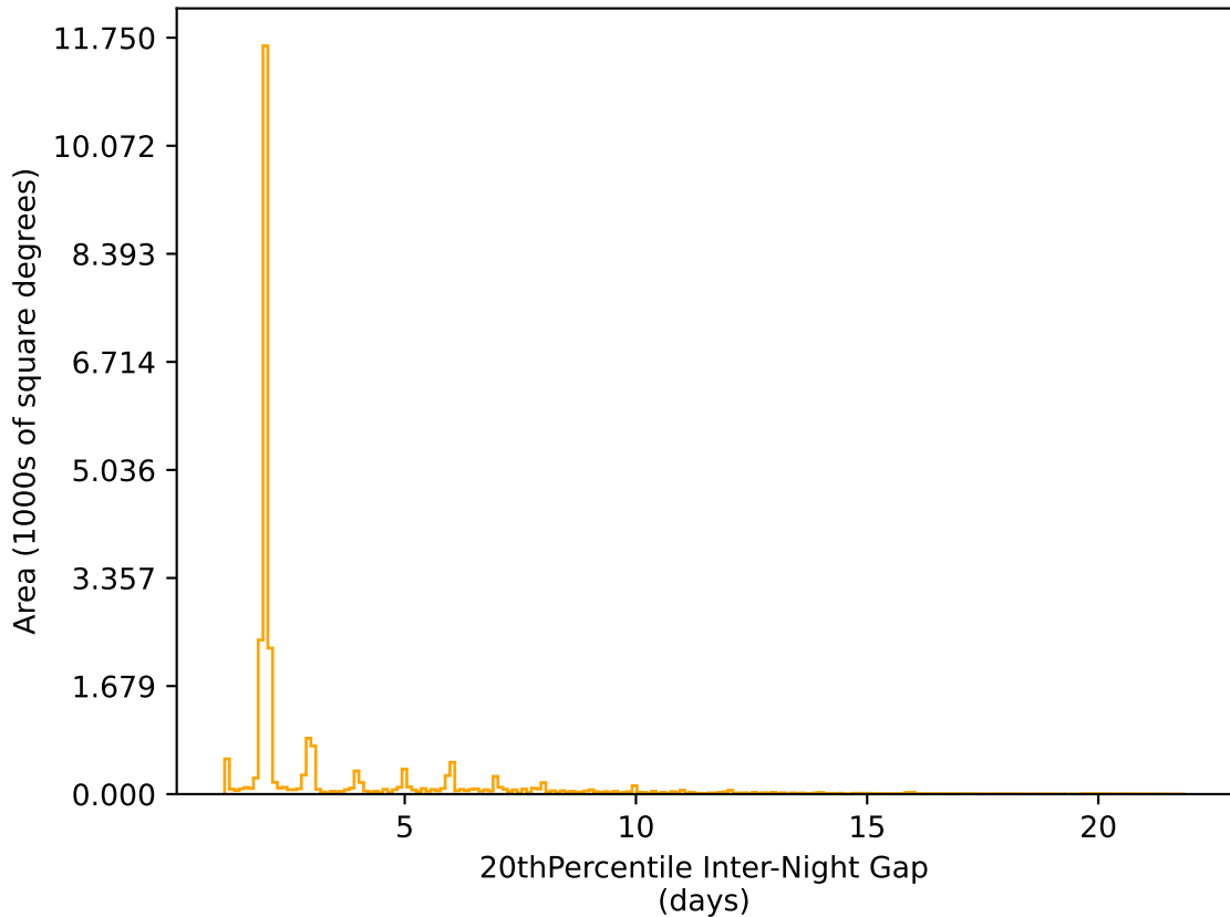
mw_roll_all_v3.3_10yrs All sky r band: 20thPercentile Inter-Night Gap
