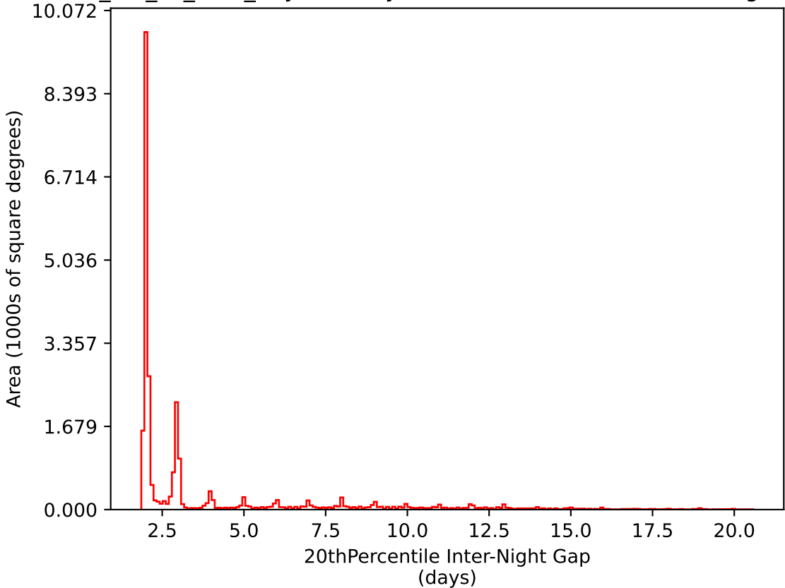
mw_roll_all_v3.3_10yrs All sky i band: 20thPercentile Inter-Night Gap
