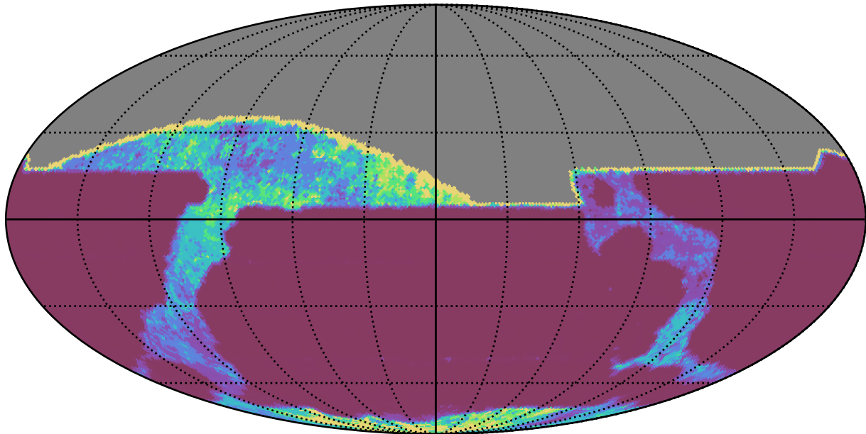
mw_roll_all_v3.3_10yrs All sky all bands: 20thPercentile Inter-Night Gap
