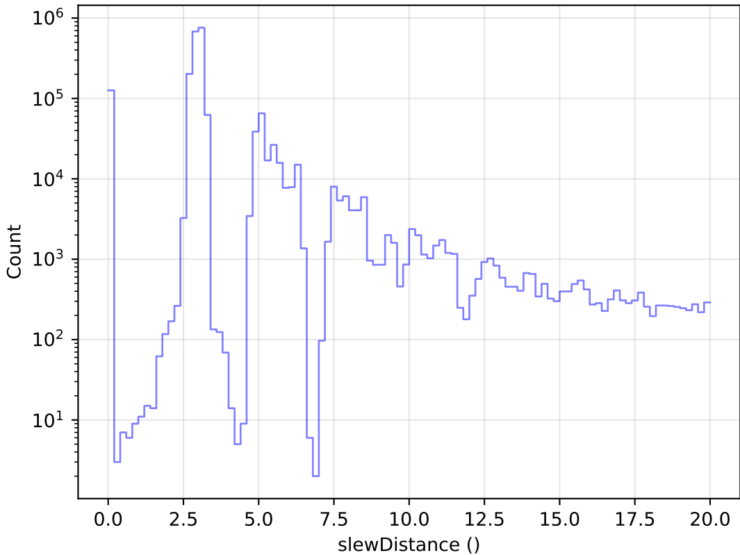
mw_roll_all_v3.3_10yrs All visits: Zoom Slew Distance Histogram
