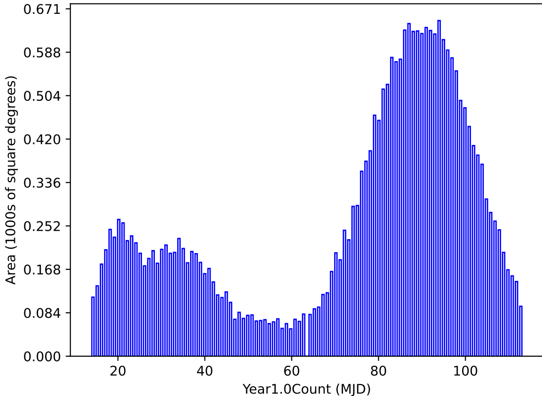
mw_roll_all_v3.3_10yrs night < 365.25: Year1.0Count
