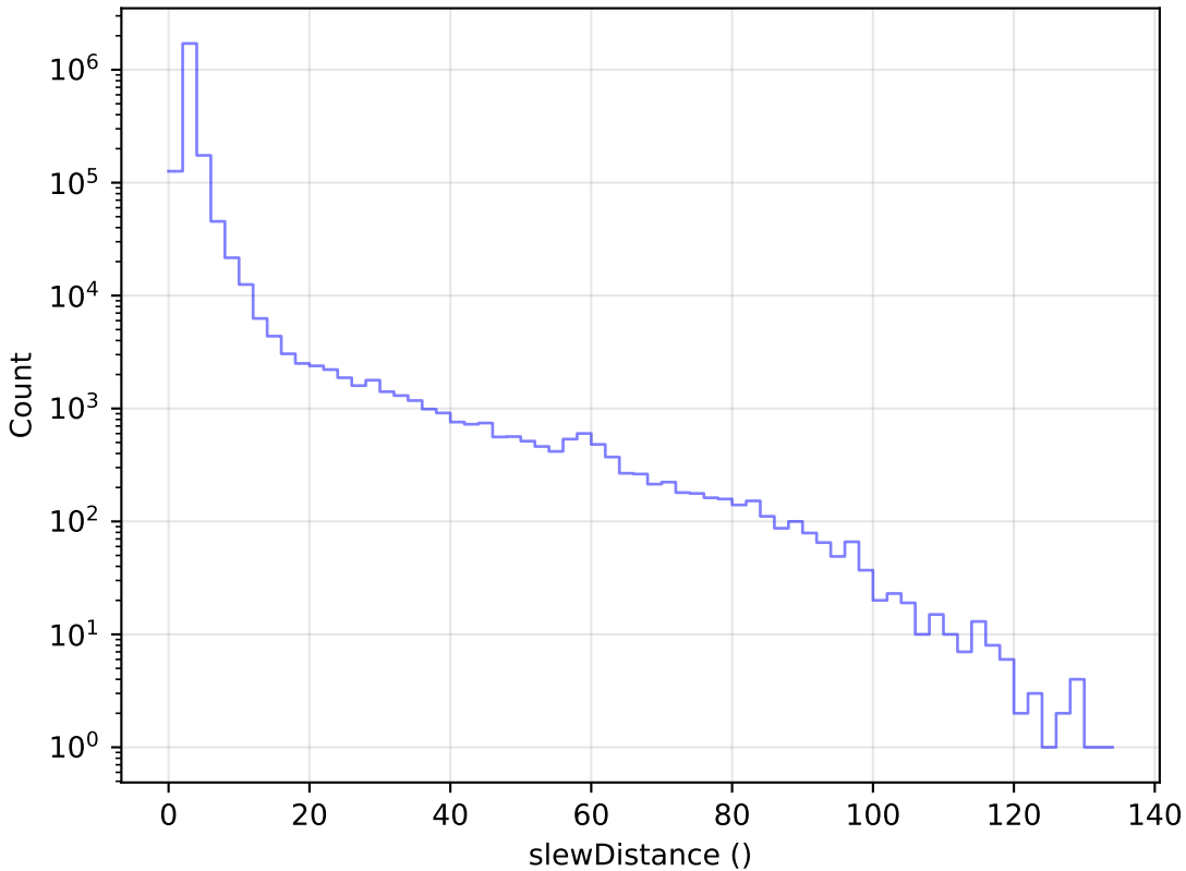
mw_roll_all_v3.3_10yrs All visits: Slew Distance Histogram
