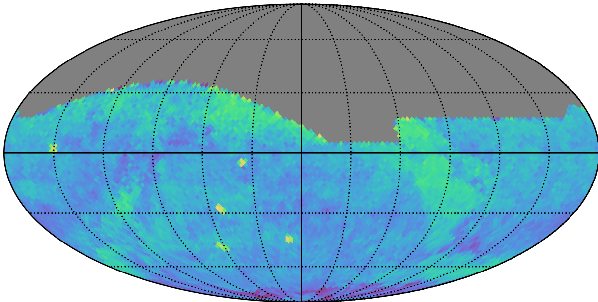
mw_roll_all_v3.3_10yrs (g or r or i): PairFraction
