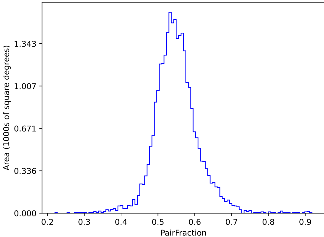
mw_roll_all_v3.3_10yrs (g or r or i): PairFraction
