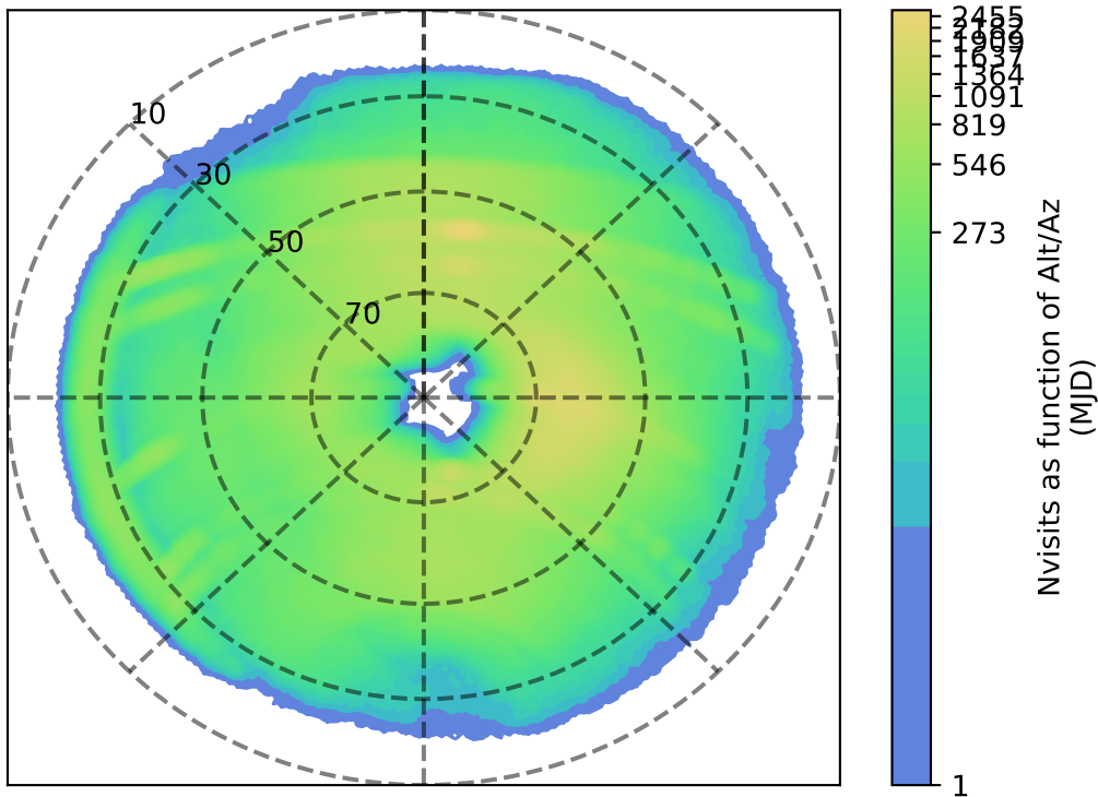
mw_roll_all_v3.3_10yrs r: Nvisits as function of Alt/Az
