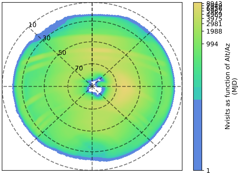
mw_roll_all_v3.3_10yrs : Nvisits as function of Alt/Az
