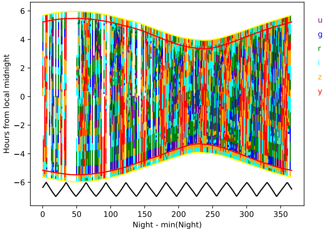
mw_roll_all_v3.3_10yrs year 6-7: Hourglass
