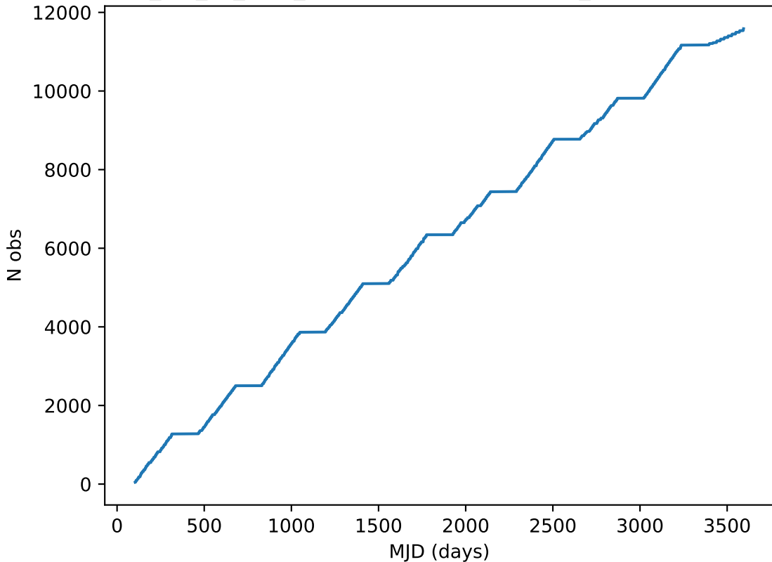
mw_roll_all_v3.3_10yrs note like DD:EDFS_b%: Cumulative
