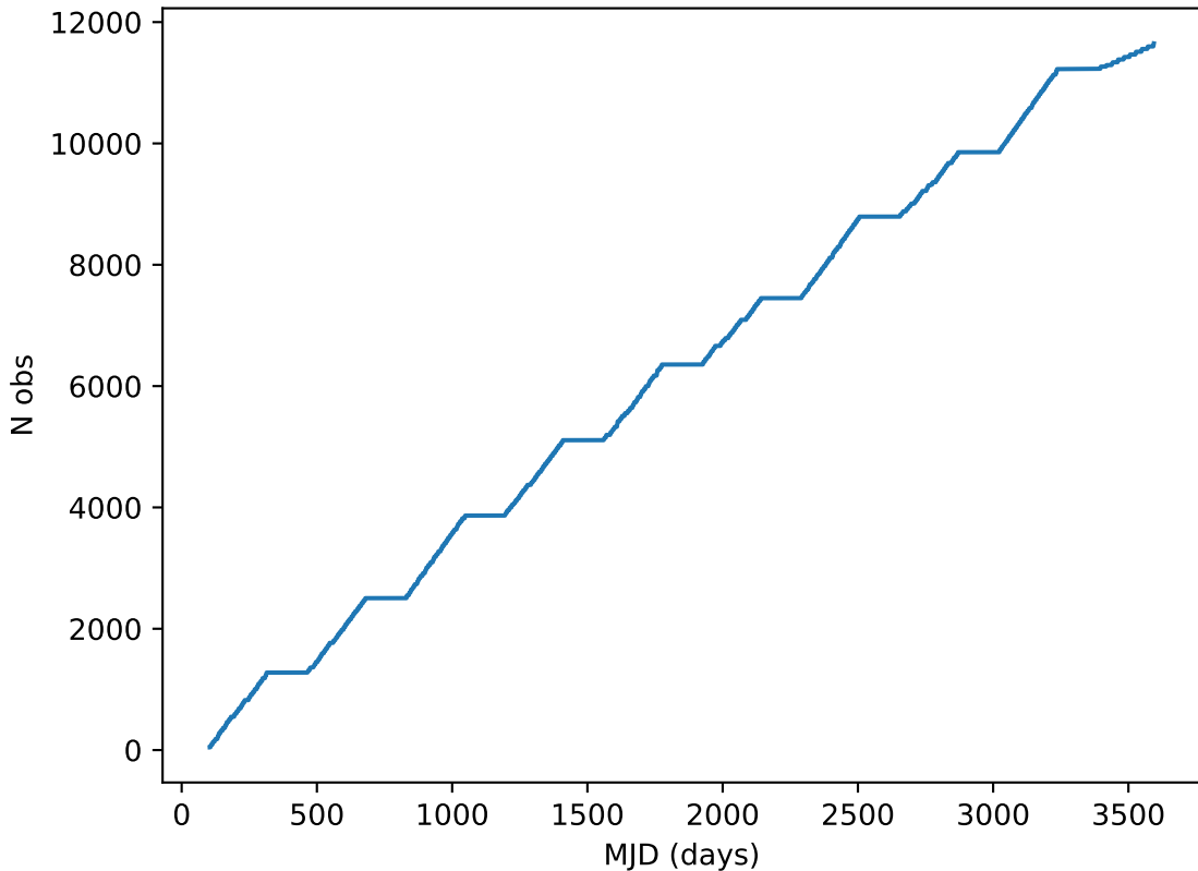
mw_roll_all_v3.3_10yrs note like DD:EDFS_a%: Cumulative
