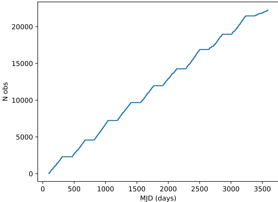
mw_roll_all_v3.3_10yrs note like DD:ECDFS%: Cumulative
