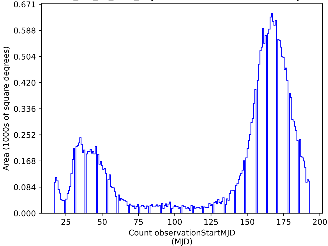
mw_roll_all_v3.3_10yrs z: Count observationStartMJD
