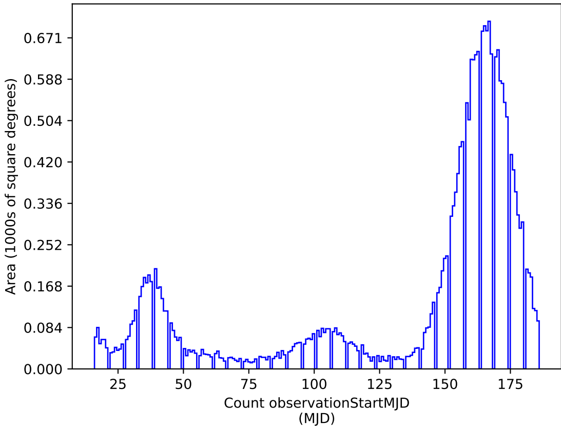
mw_roll_all_v3.3_10yrs y: Count observationStartMJD
