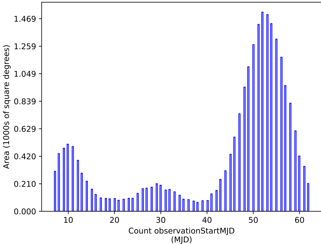
mw_roll_all_v3.3_10yrs u: Count observationStartMJD
