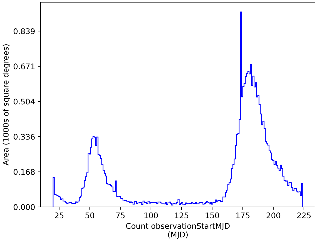
mw_roll_all_v3.3_10yrs r: Count observationStartMJD
