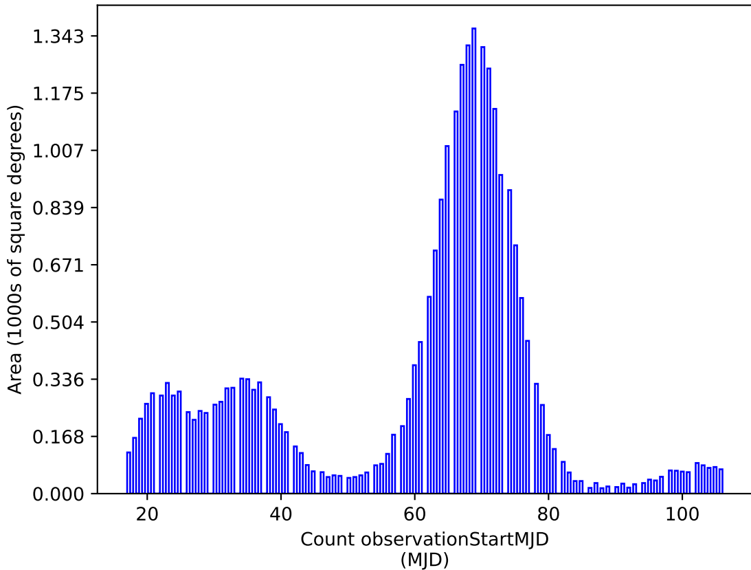
mw_roll_all_v3.3_10yrs g: Count observationStartMJD
