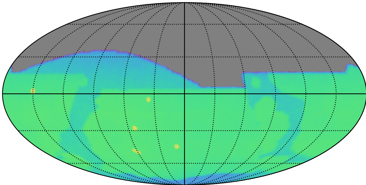
mw_roll_all_v3.3_10yrs r: CoaddM5
