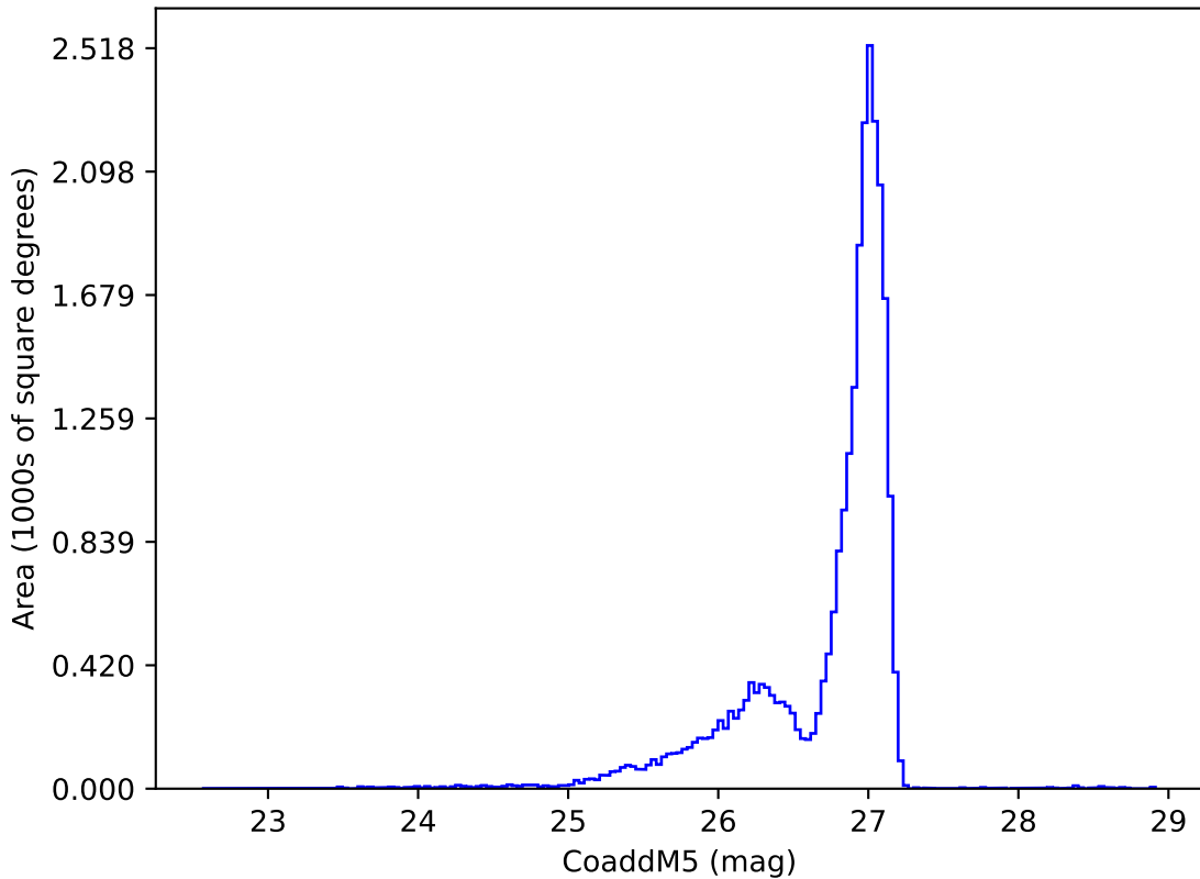
mw_roll_all_v3.3_10yrs r: CoaddM5
