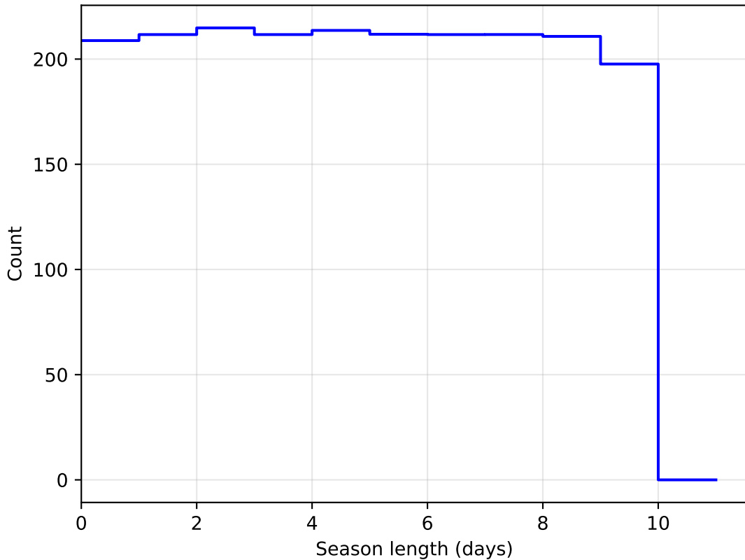
mw_roll_all_v3.3_10yrs DD:EDFS all bands: SeasonLength
