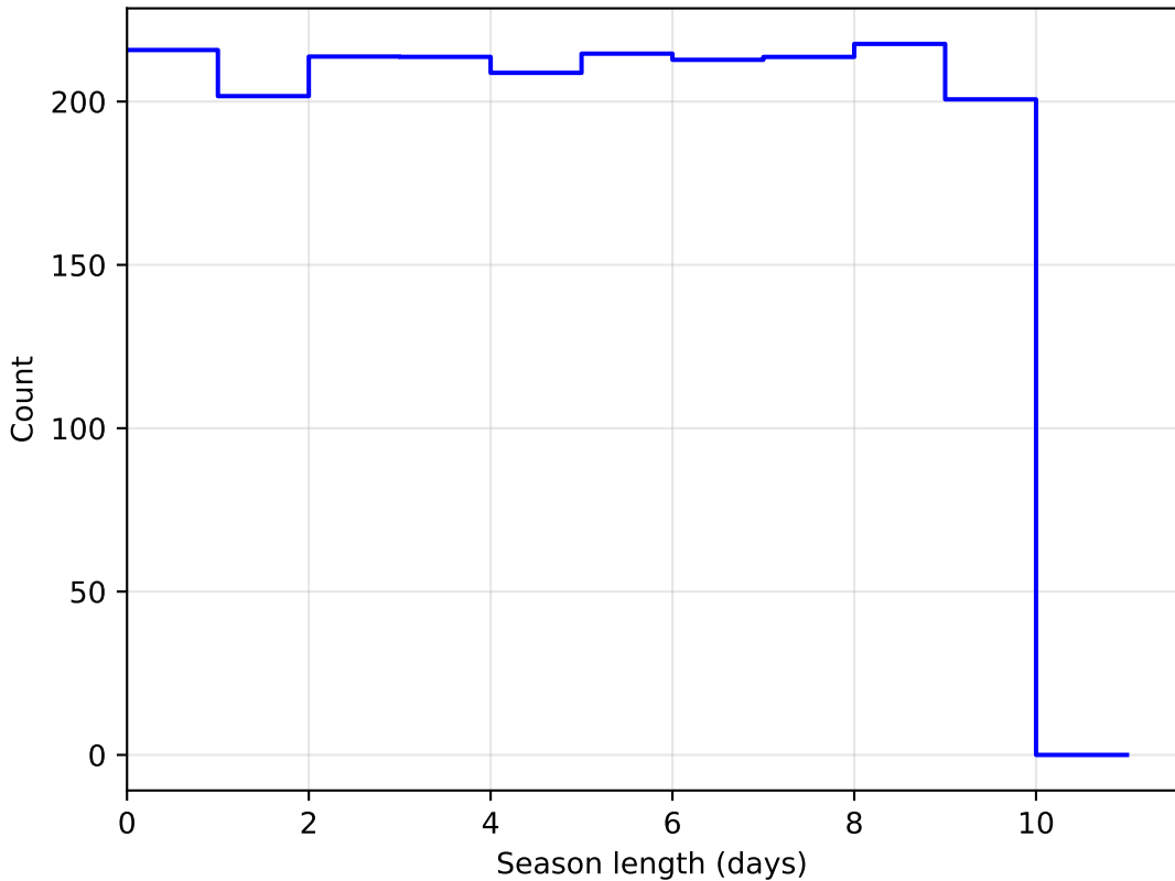
mw_roll_all_v3.3_10yrs DD:ECDFS all bands: SeasonLength
