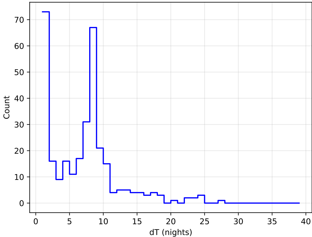
mw_roll_all_v3.3_10yrs all bands: DD:XMM_LSS Delta Nights Histogram
