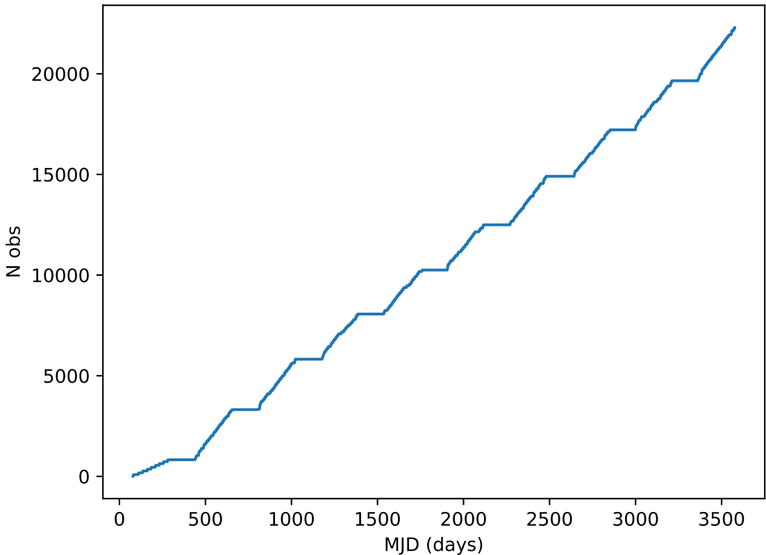
mw_roll_all_v3.3_10yrs all bands: DD:XMM_LSS Cumulative NVisits
