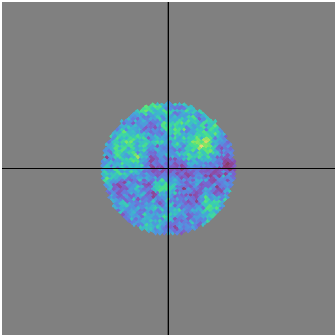
mw_roll_all_v3.3_10yrs all bands: DD:WFD NVisits
