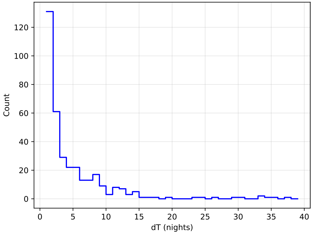
mw_roll_all_v3.3_10yrs all bands: DD:WFD Delta Nights Histogram
