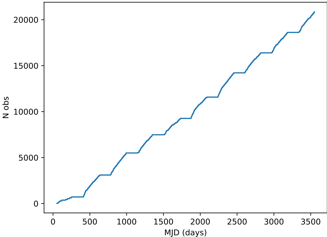
mw_roll_all_v3.3_10yrs all bands: DD:ELAISS1 Cumulative NVisits
