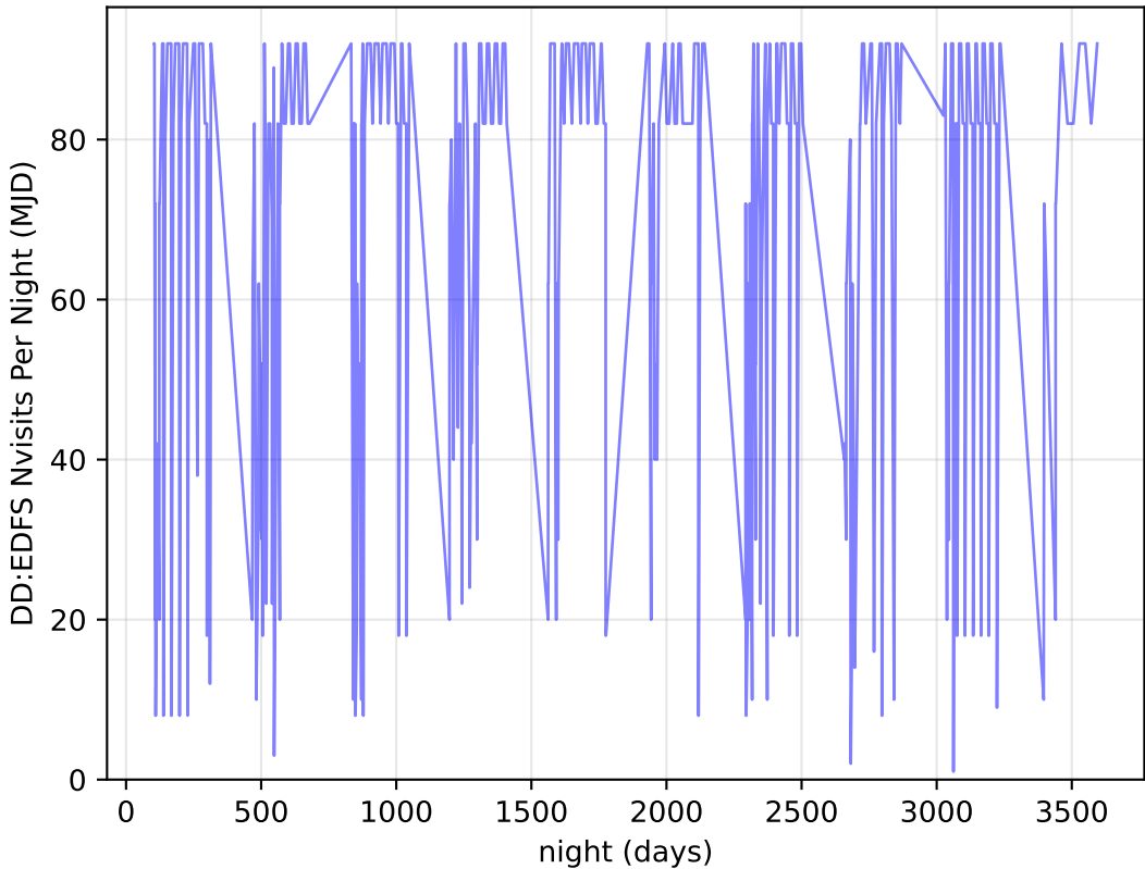
mw_roll_all_v3.3_10yrs all bands: DD:EDFS Nvisits Per Night
