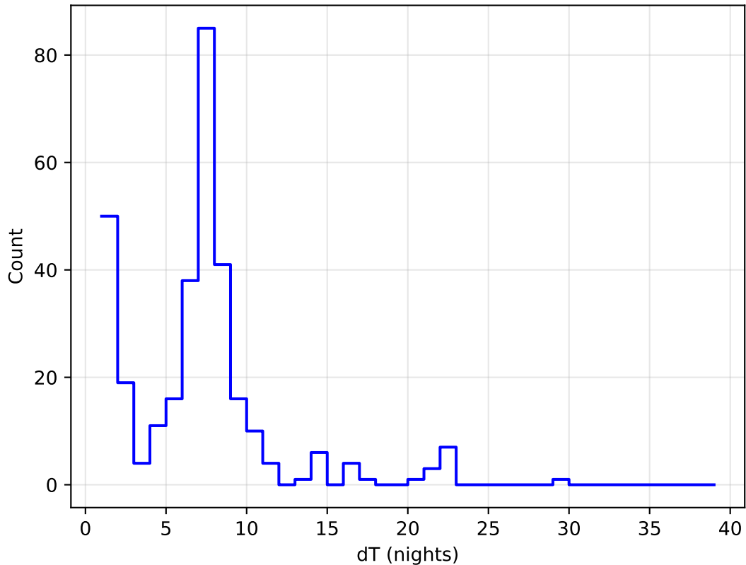
mw_roll_all_v3.3_10yrs all bands: DD:EDFS Delta Nights Histogram
