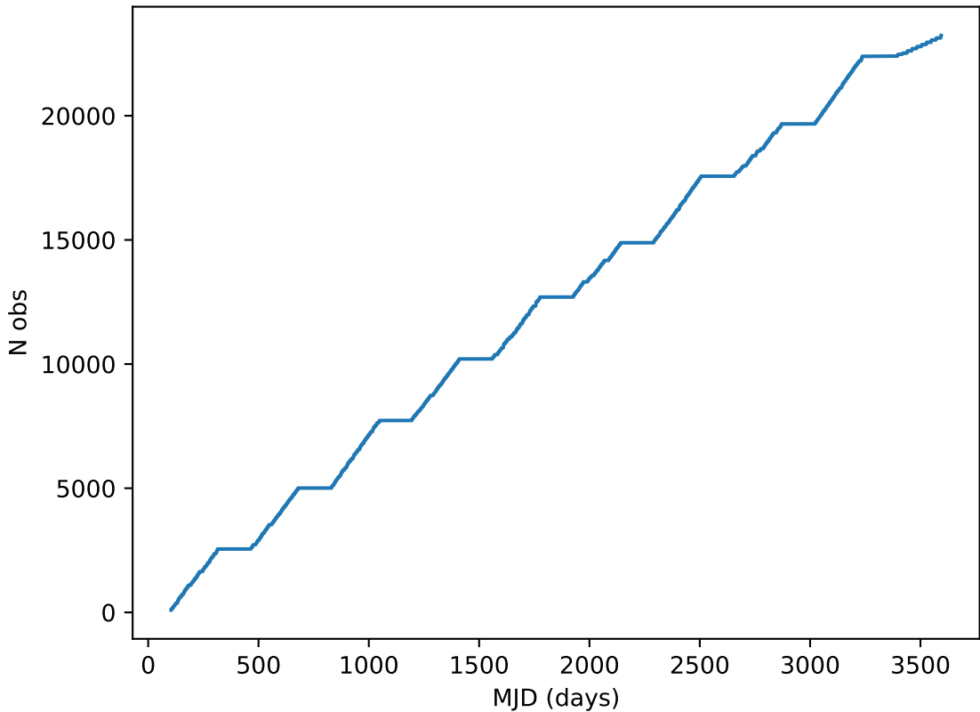
mw_roll_all_v3.3_10yrs all bands: DD:EDFS Cumulative NVisits
